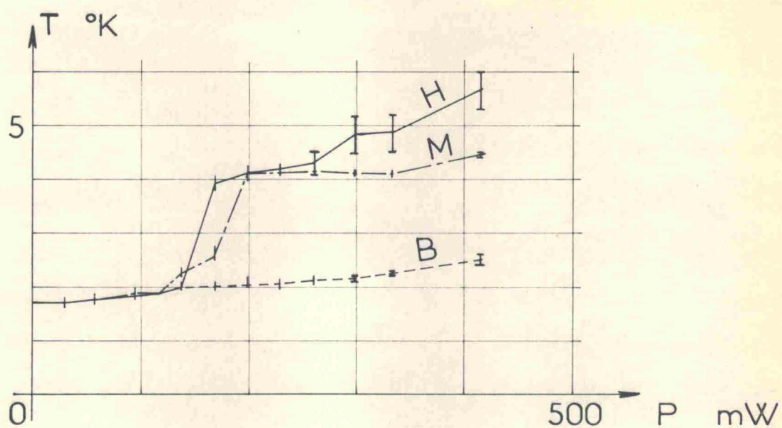
FIG.9 : Superfluid helium T = 1.7 K ; p = 1 atm
