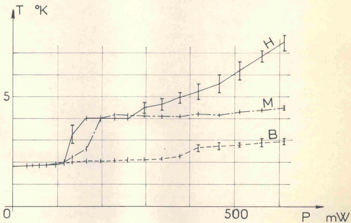
FIG.10 : Superfluid helium T = 1.8 K ; p = 1 atm
